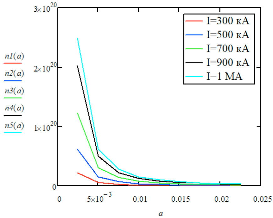
Fig 1 – Changes in the concentration of electrons from the distance between the electrodes for different values of current
